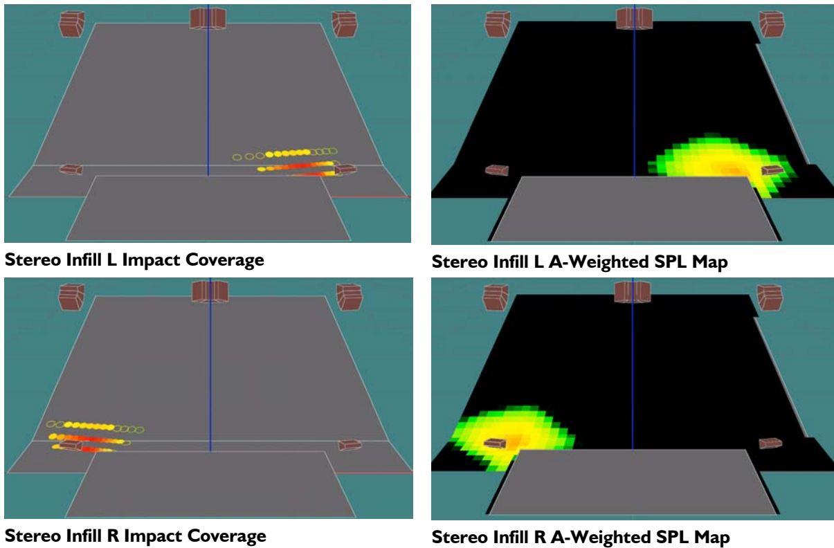
Figure 24: Impact coverage and A-weighted SPL mappings for the theatrical sound design example of Figure 19
