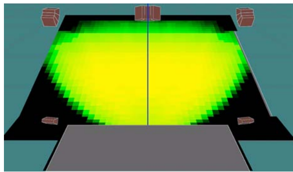
Centre Cluster A-Weighted SPL Map
