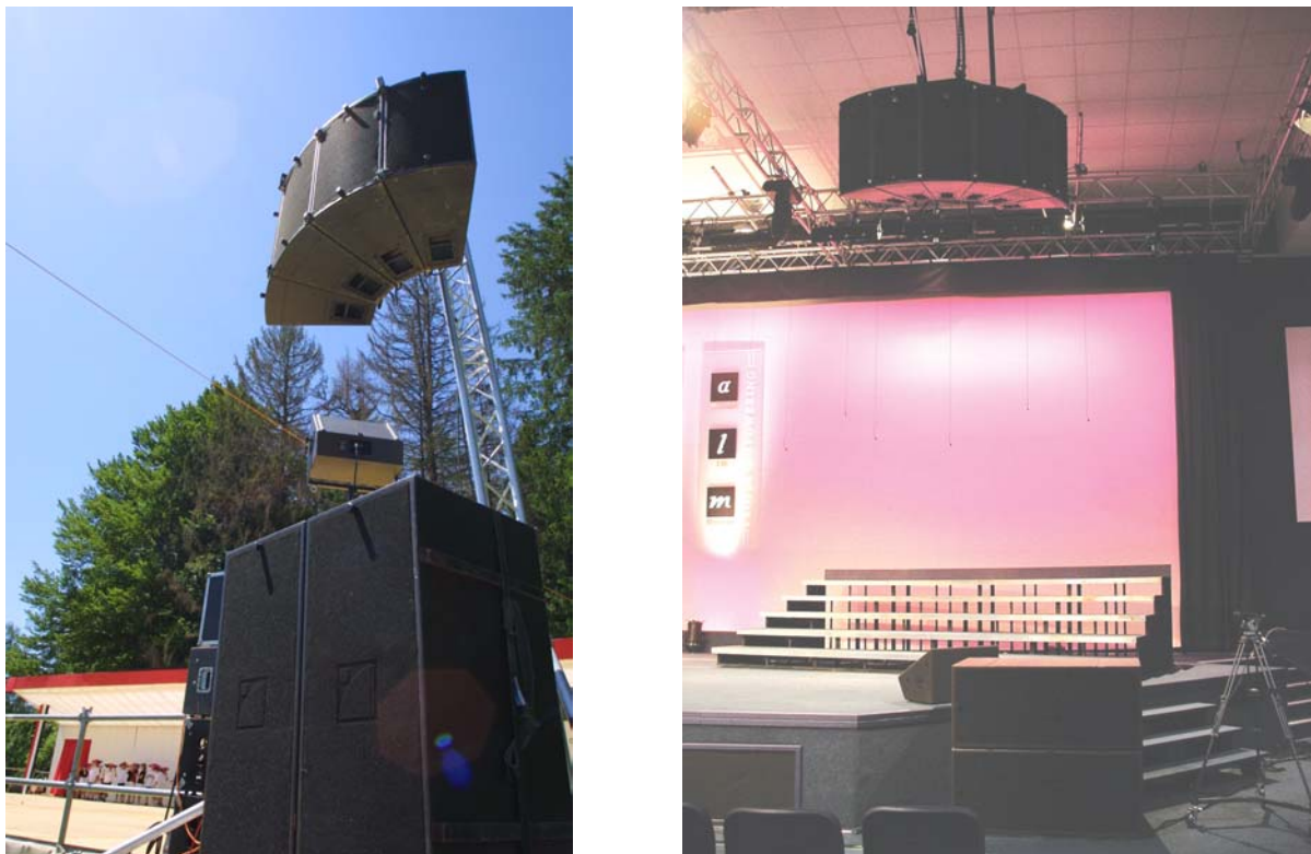
Figure 26: Single Row ARCS Array Examples
